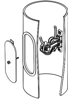
Internal Cam Cleat and Handhole Door
